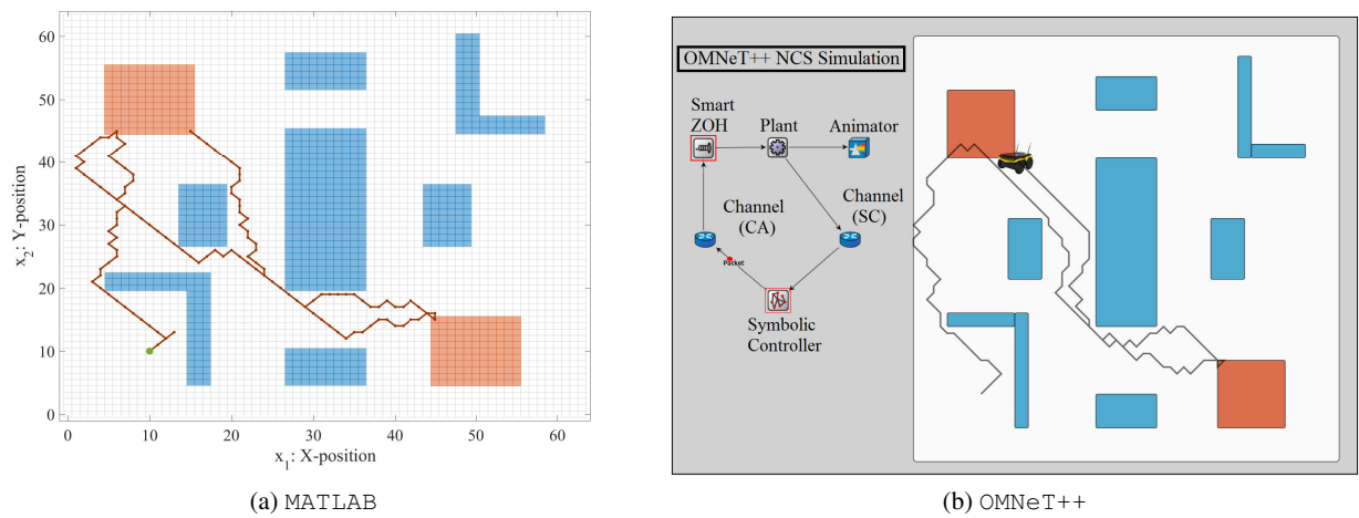
Figure 5: Closed-loop simulation of the robot in MATLAB and in OMNeT++. Two target sets are represented by red boxes. Nine obstacle sets are represented by blue boxes.
