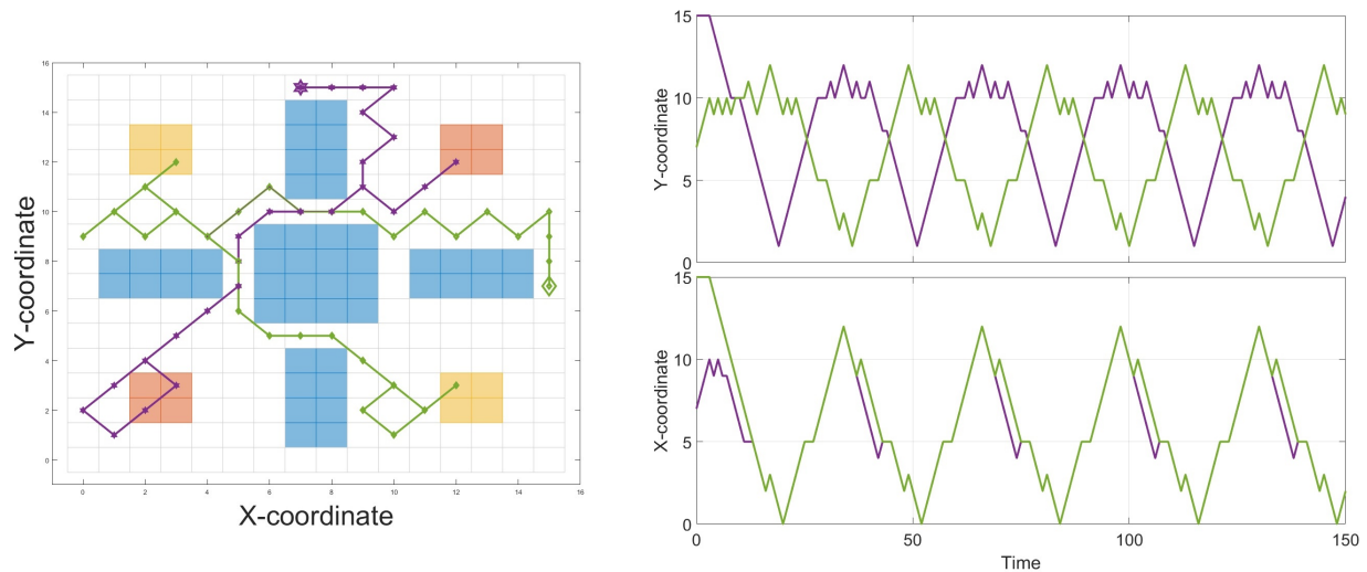
Figure 7: Closed loop simulation of the two robots example in MATLAB.
