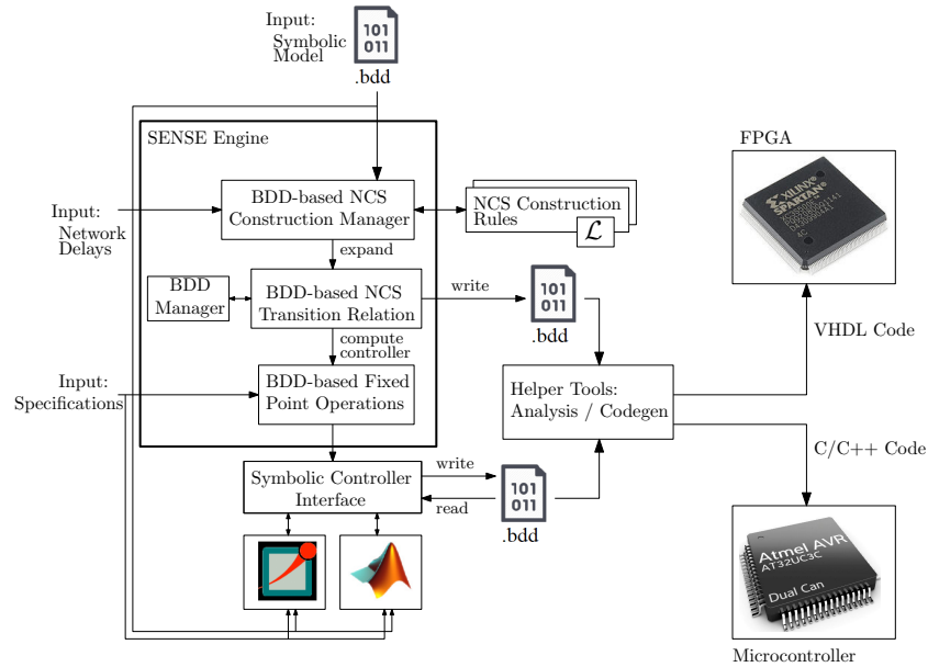
Figure 3: Work flow inside SENSE: from specifications to ready-to-implement source codes.
