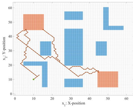
(a) MATLAB
